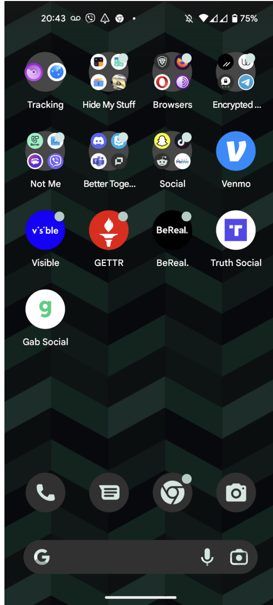
Figure 6. Home Screen 2.
