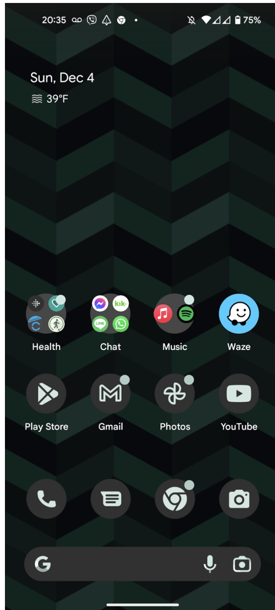
Figure 1. Home Screen 1
